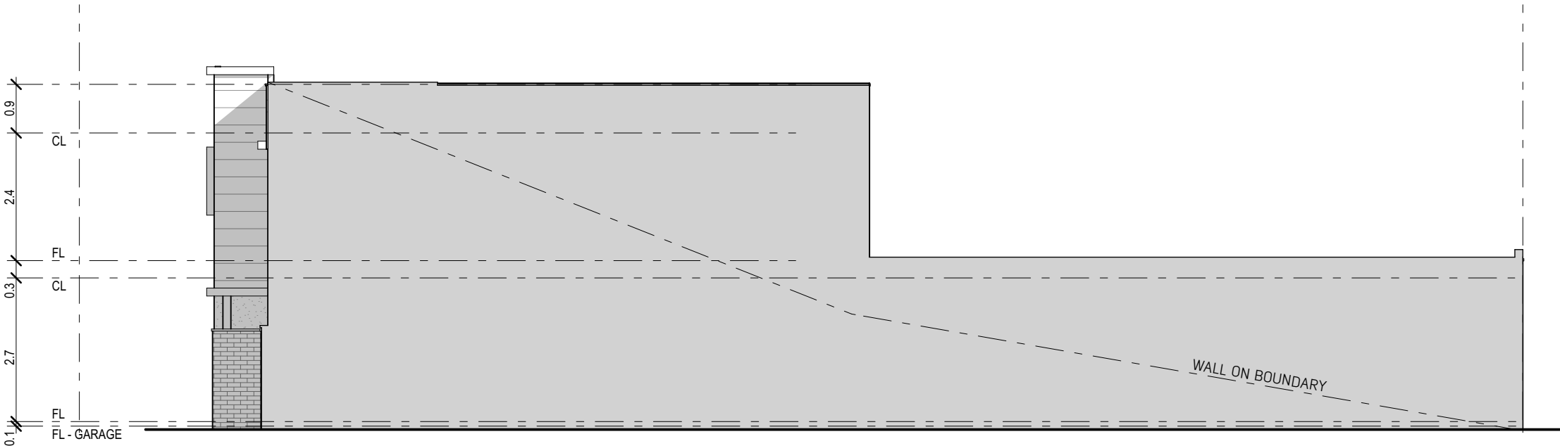
TYPE P - FACADE A 02. 1:100
