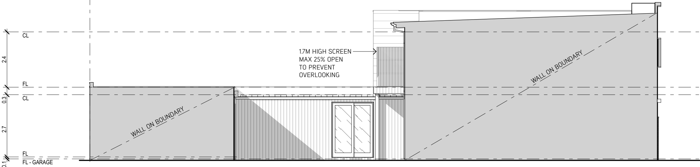
TYPE P - FACADE A 02. 1:100
