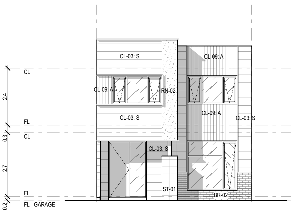
TYPE P - FACADE B 01. 1:100
