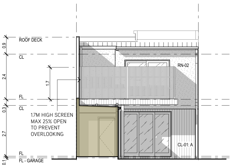
TYPE P - FACADE A 05. 1:100
