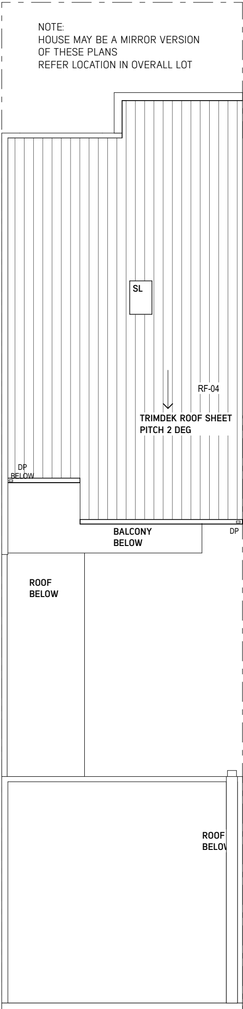
ROOF PLAN
