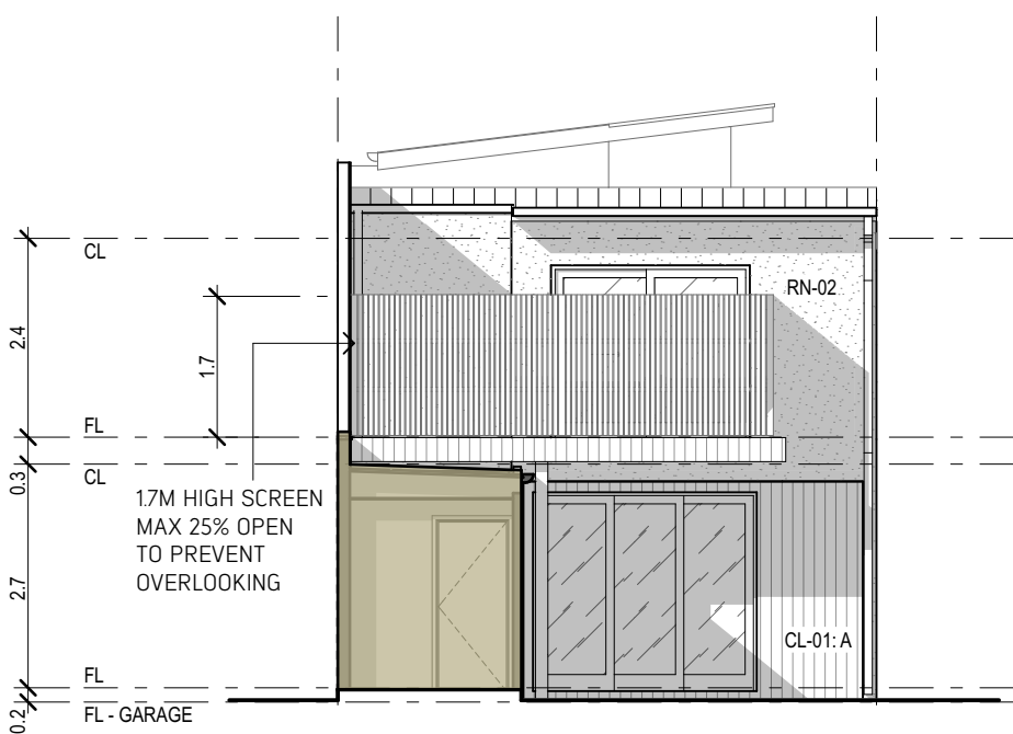
TYPE P - FACADE C 05. 1:100
