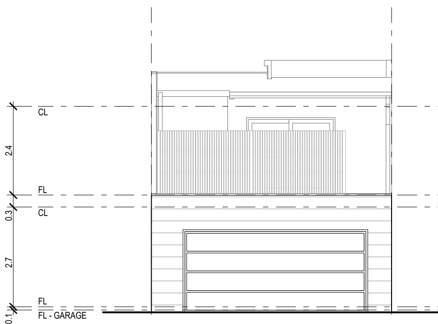
TYPE P - FACADE A 03. 1:100
