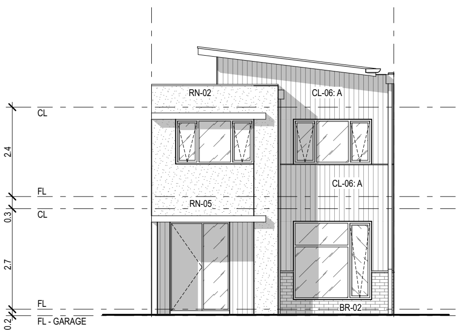
TYPE P - FACADE C 01. 1:100
