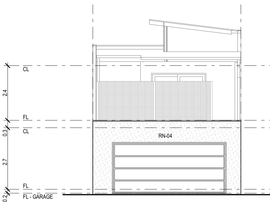
TYPE P - FACADE D 03. 1:100
