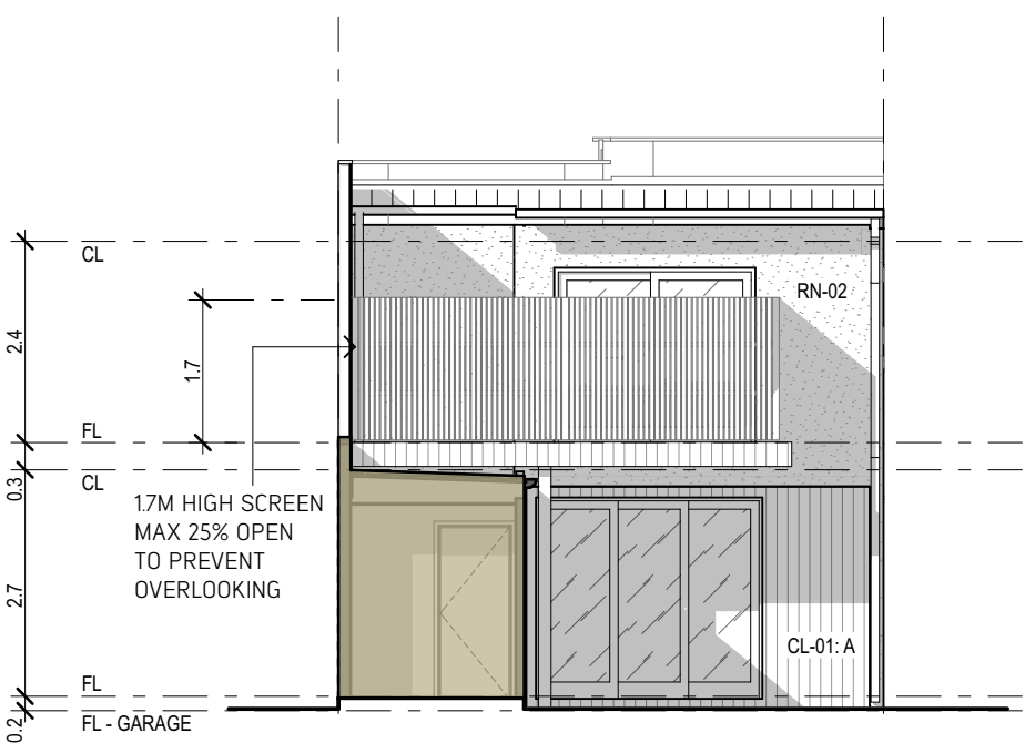
TYPE P - FACADE B 05. 1:100
