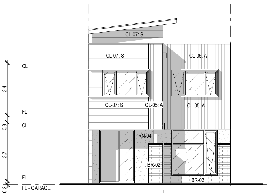
TYPE P - FACADE D 01. 1:100
