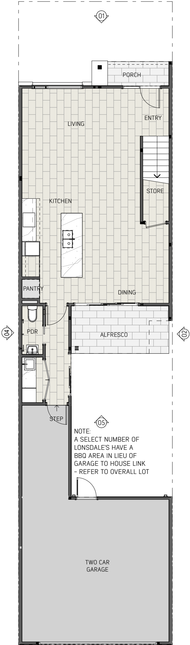
GROUND FLOOR
