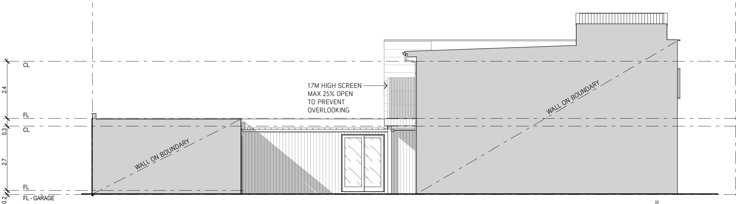
TYPE P - FACADE D 01. 1:100
