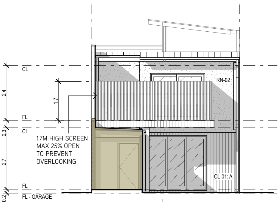
TYPE P - FACADE D 05. 1:100
