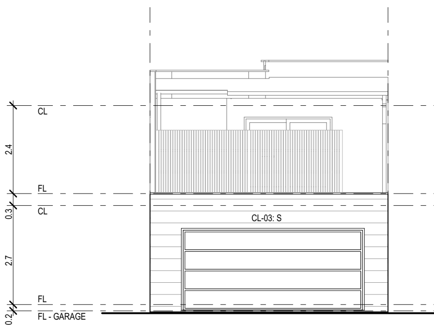
TYPE P - FACADE B 03. 1:100
