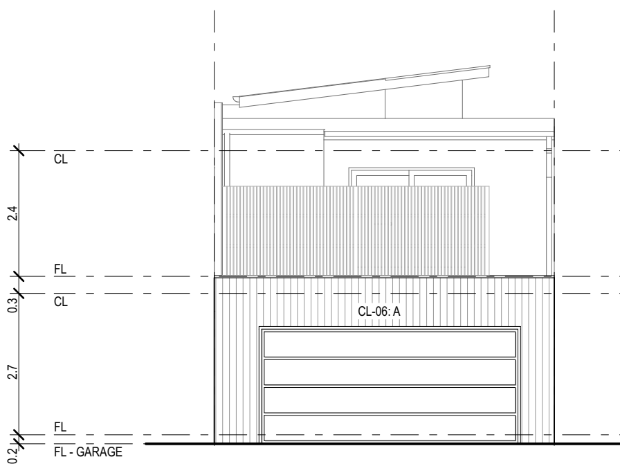
TYPE P - FACADE C 03. 1:100
