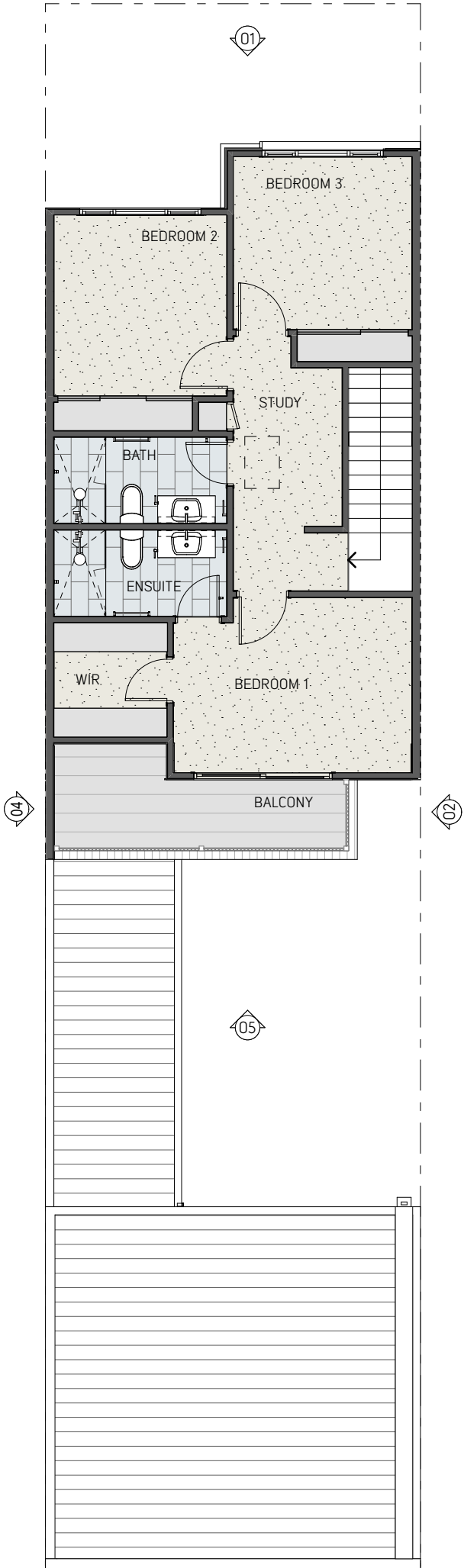
FIRST FLOOR
